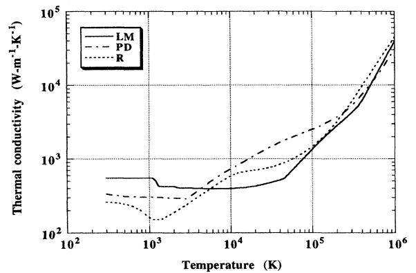
FIG. 4. Thermal conductivity as a function of temperature for aluminum at solid density. The data for Perrot and Dharma-wardana's model are obtained using the Wiedemann-Franz law.
